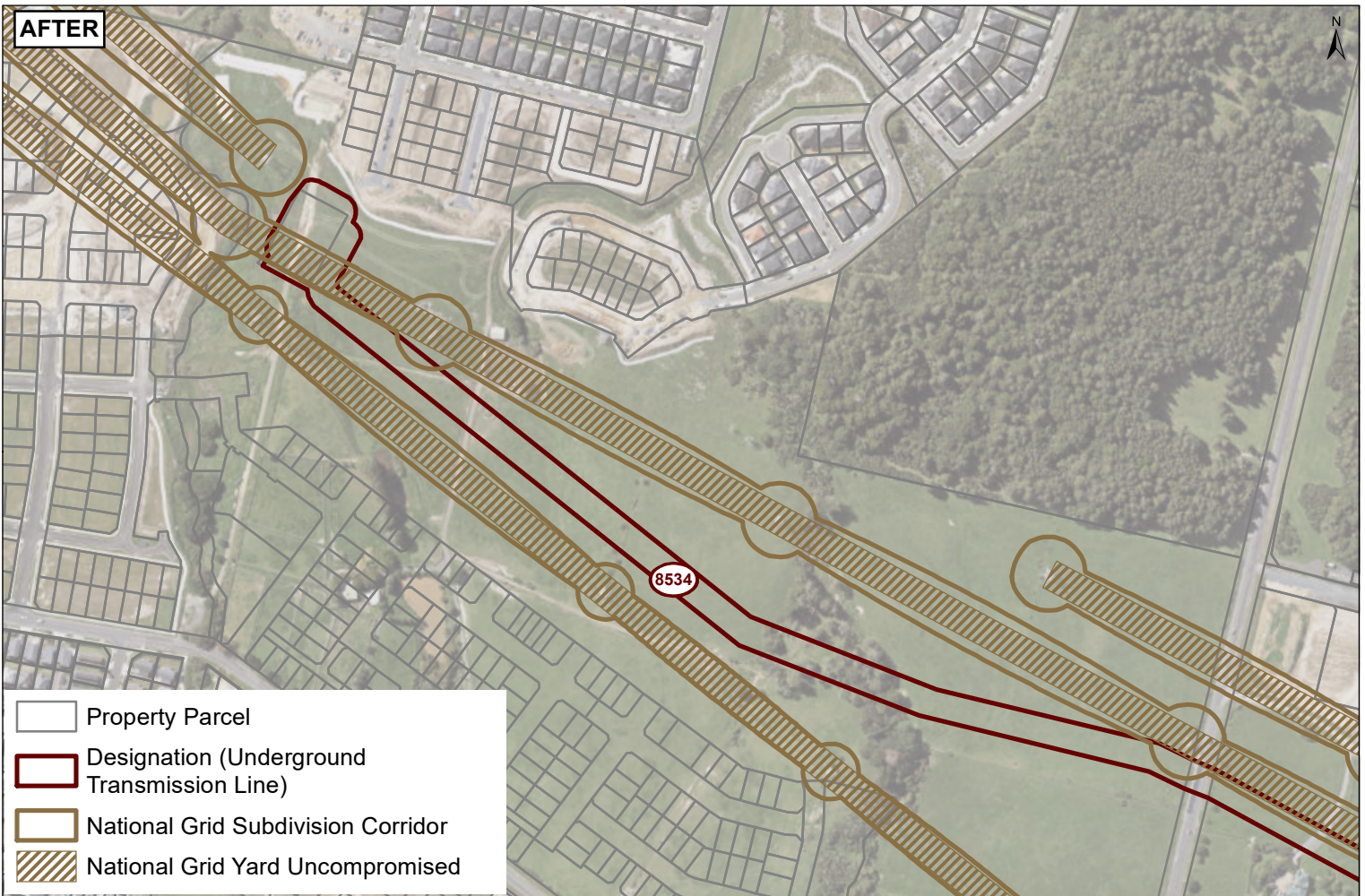
Figure 1 – Section of National Grid Overlay (OTA-WKM-A Line) to be removed
